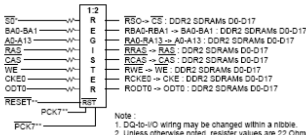
Signals for Address and Command Parity Function (M393T2950CZA)
